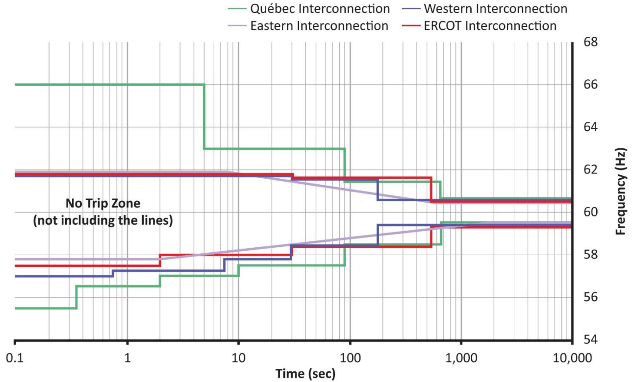
Figure 2.4: PRC-024-2 Frequency Ride-Through Curves
