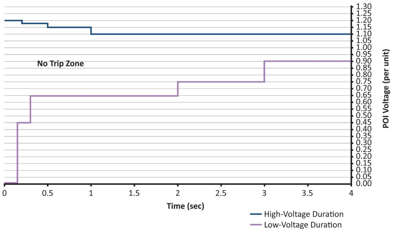
Figure 2.5: PRC-024-2 Voltage Ride-Through Curves
